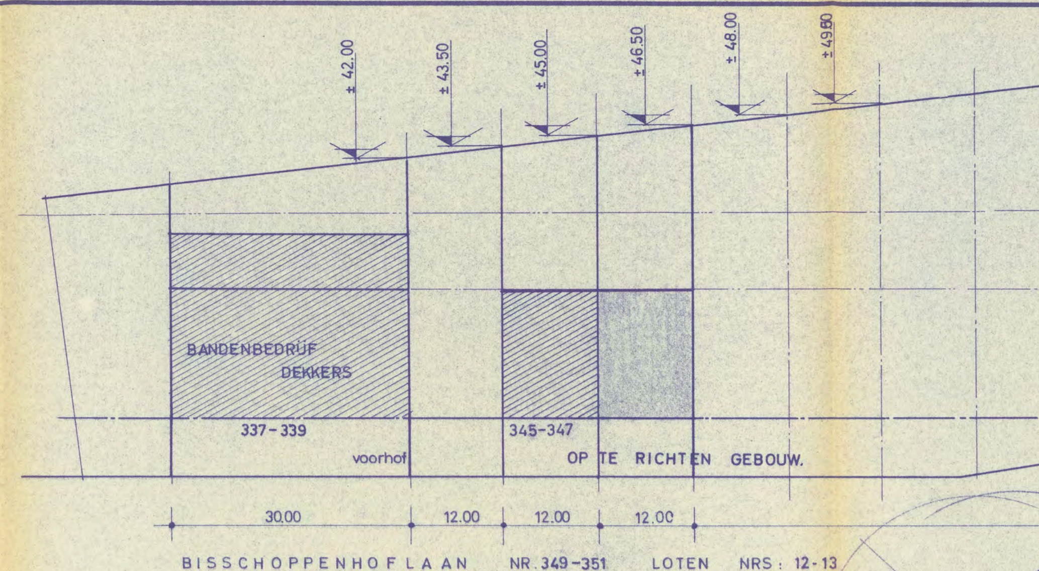
inplantingsplan
